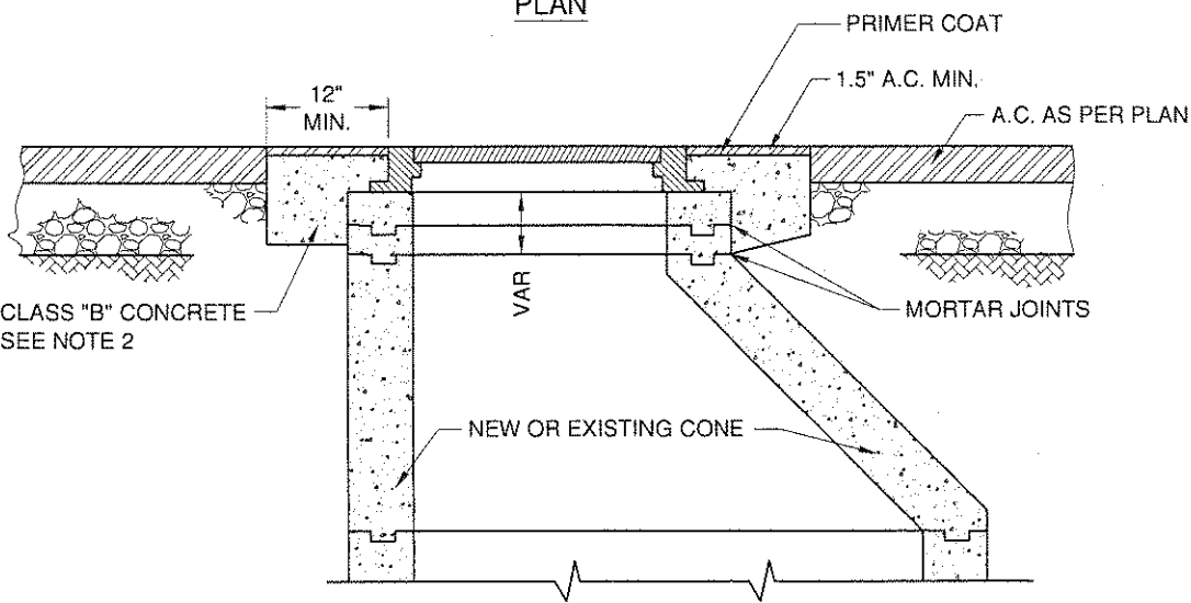
CROSS-SECTION
