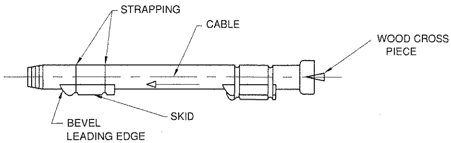
SIDE VIEW OF C-900 PVC PIPE ON SKIDS
