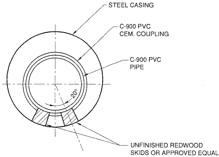
CROSS SECTION OF C-900 PVC INSTALLED IN STEEL CASING
