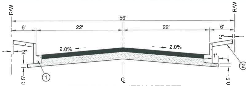
RESIDENTIAL ENTRY STREET
