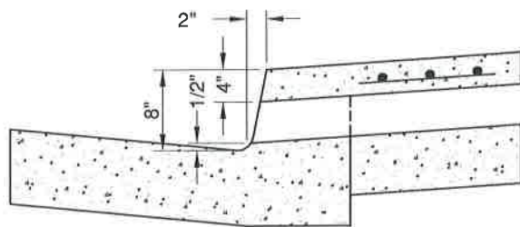
SECTION A-A (8" CURB FACE)
