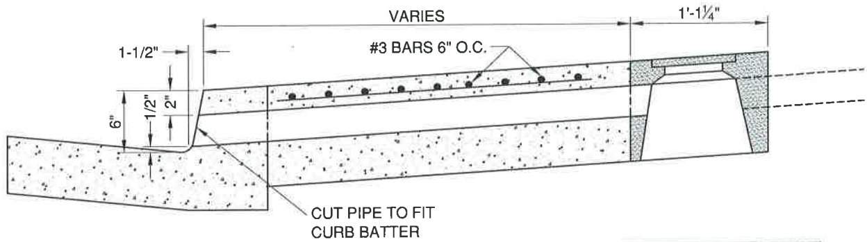
SECTION A-A (6" CURB FACE)
