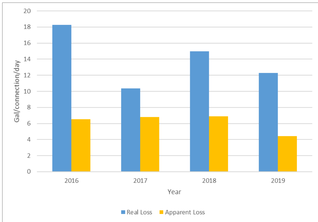
Figure 4-3: Water Loss Performance Indicator for CY2016 - 2019
