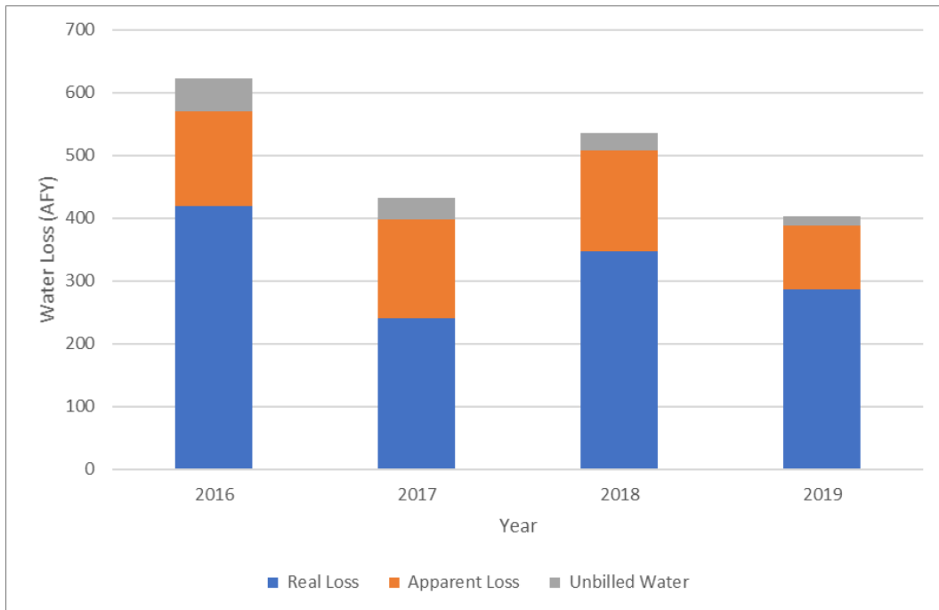
Figure 4-2: Water Loss Audit for CY2016 – 2019
